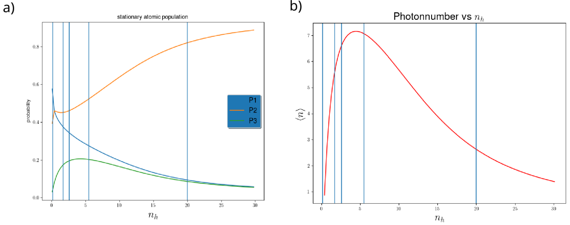
Figure 3: In Fig. 3a the probability for an atom to stay in a state |1\rangle , |2\rangle or |3\rangle vs n_h is plotted. With an increasing n_h P2 increases as well until a population inversion happens P2 > P1 . The probability for P1, P2, P3 is in the region of n_h = 5 well distributed. The parameters for the first plot are n_c = 0.02, n_f = 0.02, \kappa = 0.01\gamma_h . The blue lines mark the values of n_h for which the Wigner functions are plotted. In Fig. 3b we see, the expectation value of the photon number versus n_h .
